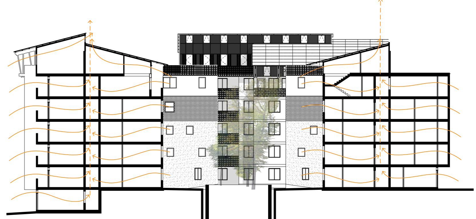
Natural Ventilation
