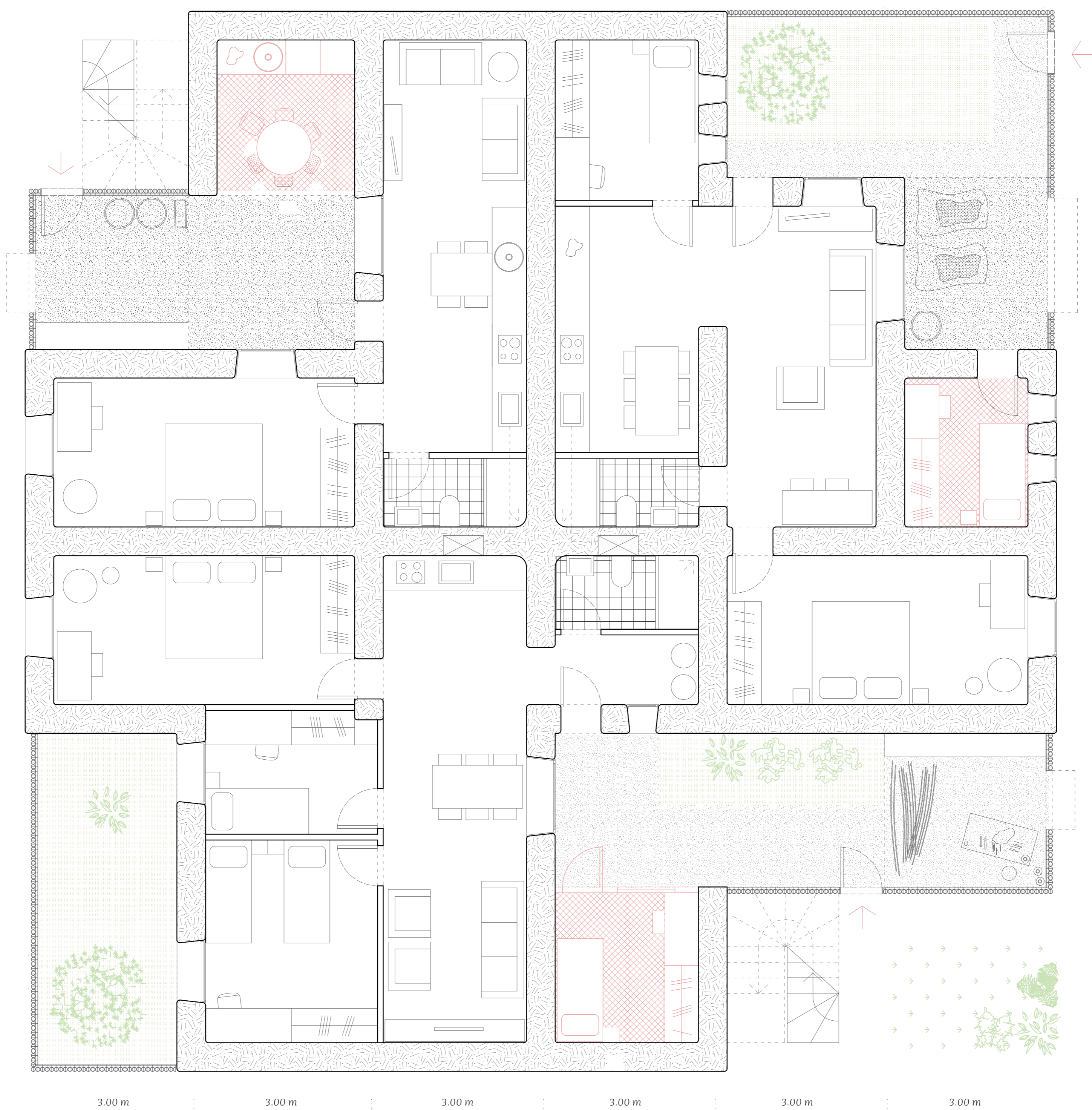
Middle/high-income group 5 private courtyard houses (40 to 100 sqm), +0.00
