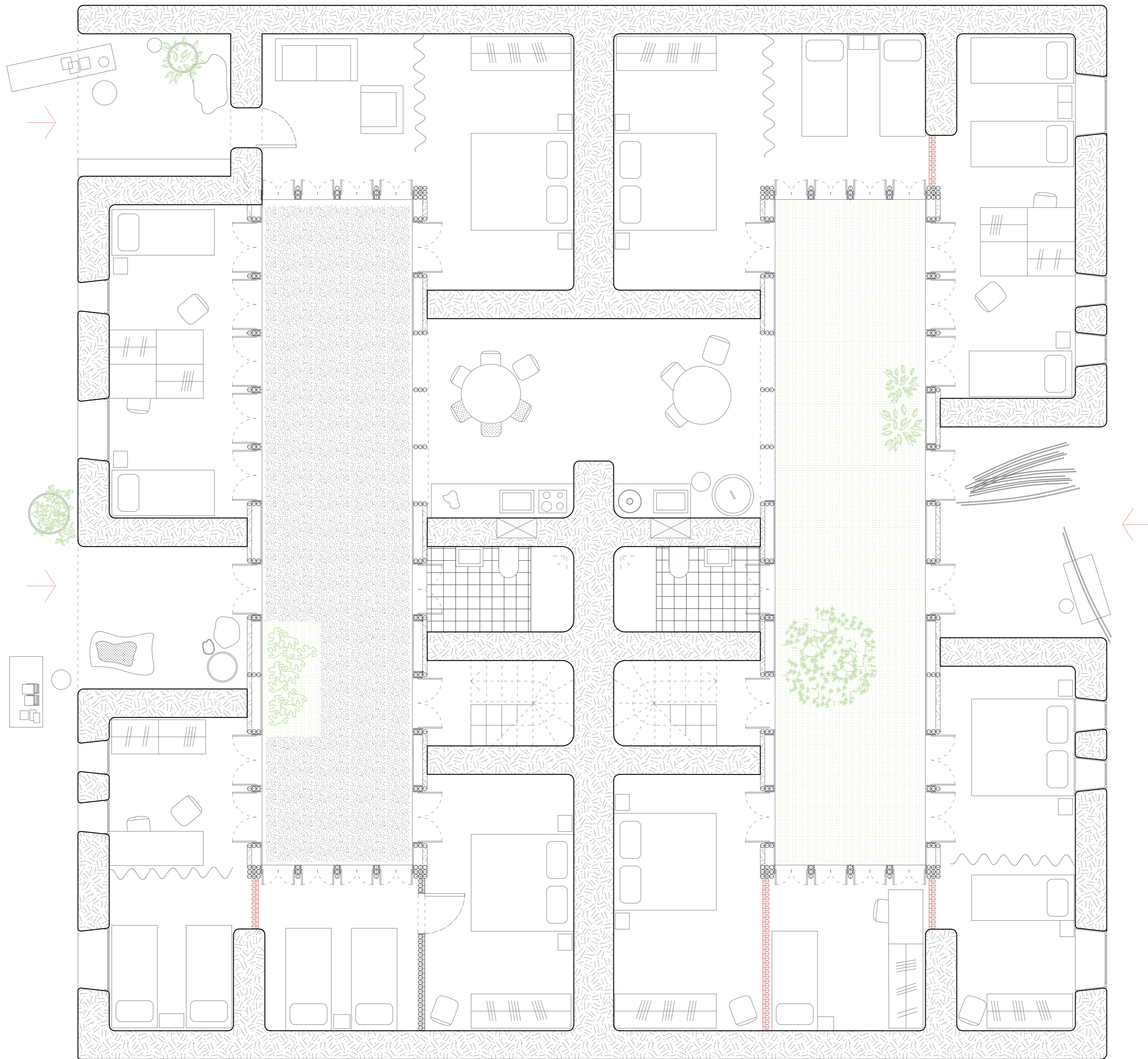
Middle/high-income group 5 private courtyard houses (40 to 100 sqm), +0.00
