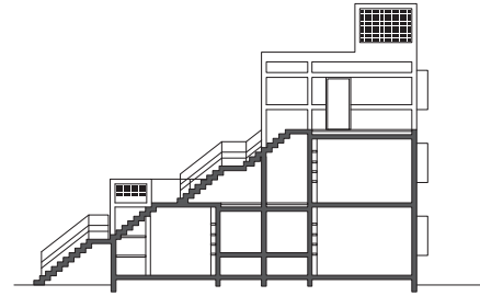
Section (A2)
