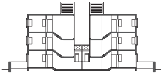
Section (A1/B1/C1)
