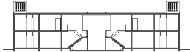
Section F2/F3
