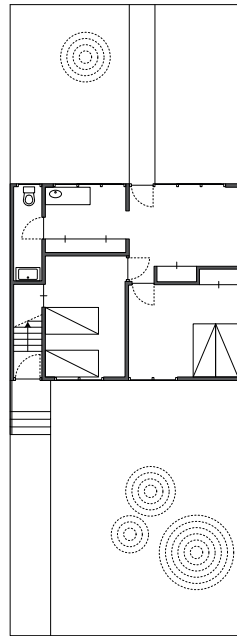
Type B08 Ground floor and first floor
