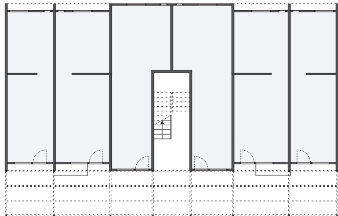
Apartments: ground floor with commercial spaces (below), typical ground floor (middle) and typical floor (above)
