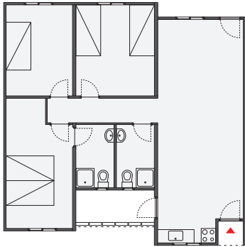
Single-storey single-family dwellings (type Acácia)
